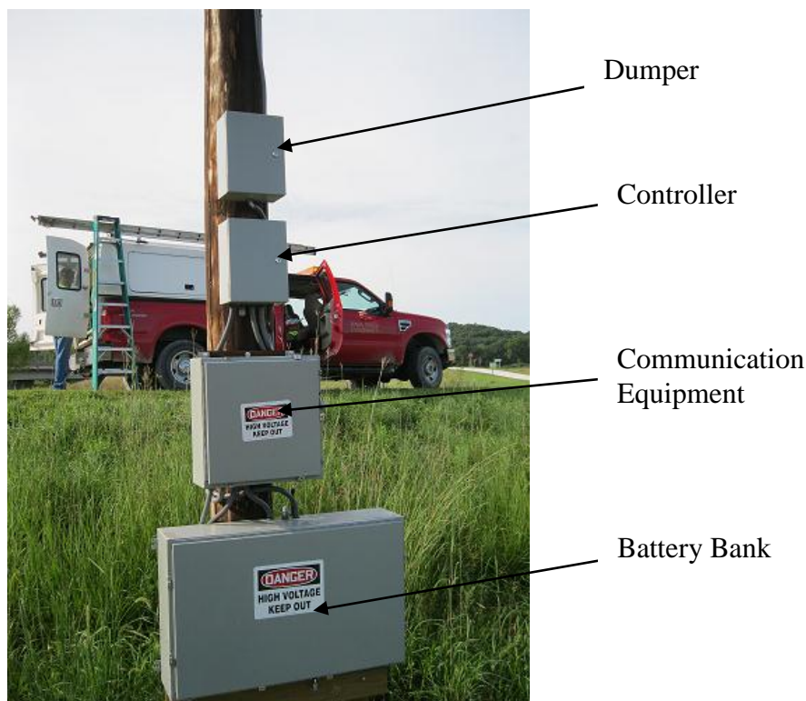
Figure 32: Hogback Enclosure Set Up
