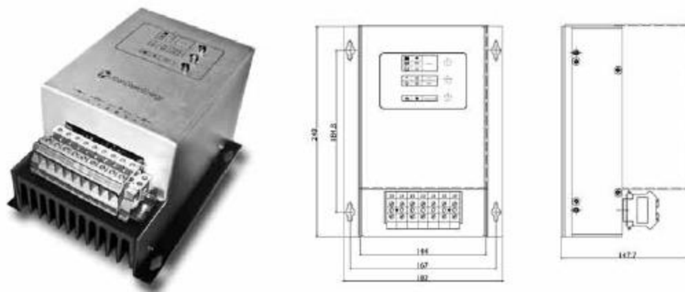
Fig. 1: UGE-600-OGC dimensions (all units in mm)
