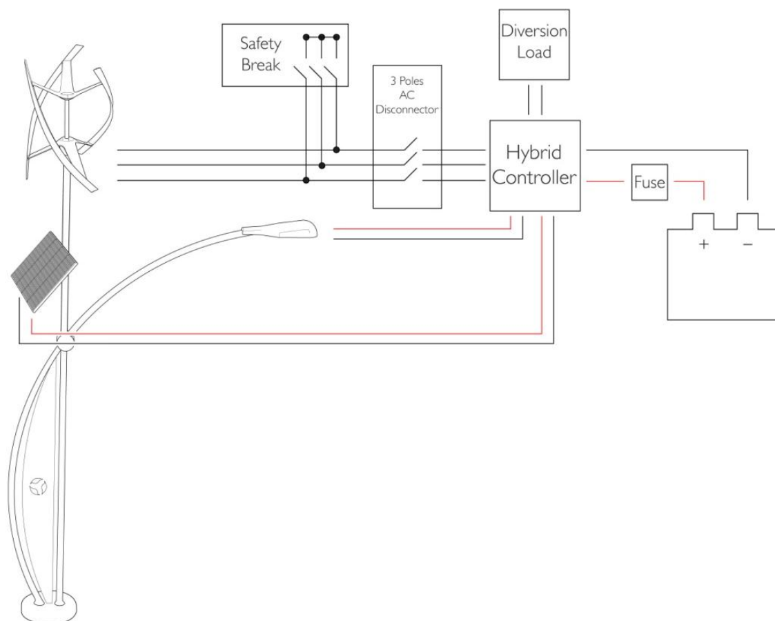
Figure 35: Wiring Diagram for an Off-Grid System with Solar and Wind Power
